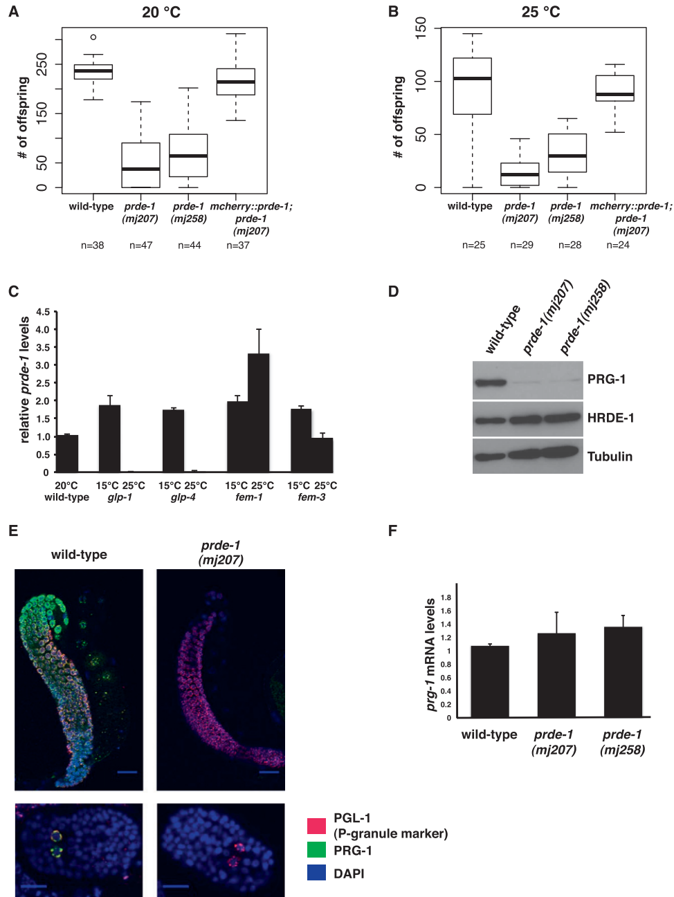
Figure 2. PRDE-1 is a nuclear germline protein required for normal fertility. (A,B) Progeny counts in wild-type and prde-1 mutant animals and one prde-1 rescue line at 20°C and 25°C. (n) Number of parental adults used (see Supplemental Fig. S2A,B). (C) prde-1 is expressed in the male and female germline of C. elegans . qRT-PCR depicts changes in prde-1 mRNA levels in temperature-sensitive germline mutants at the permissive (15°C) restrictive (25°C) temperatures. At the restrictive temperature, glp-1 and glp-4 are germlineless, fem-1 is feminized, and fem-3 is masculinized. Transcript levels are normalized to actin-3 . For Ct = undetermined, values were set to the maximum Ct of 40. Error bars are the SEM of two biological replicates. (D, top) Western blot showing down-regulation of PRG-1 in prde-1 mutants as compared with wild-type. HRDE-1, a germline-expressed nuclear Argonaute protein, is shown as a control for the presence of the germline (middle), and tubulin is shown as a general loading control (bottom). (E) Immunofluorescence staining of wild-type and prde-1 (mj207) mutant animals for PRG-1 (green), the P-granule marker PGL-1 (OIC1D4) (red), and DNA (DAPI, blue). Distal germlines are shown on top (40× magnification; bar, 20 μm), and embryos with primordial germ cells are at the bottom (60× magnification; bar, 10 μm). (F) qRT-PCR of prg-1 mRNA levels in wild-type and prde-1 mutant animals. Data are normalized to the germline-expressed gene cgh-1 . Error bars are SD; data are relative to a wild-type standard curve.
